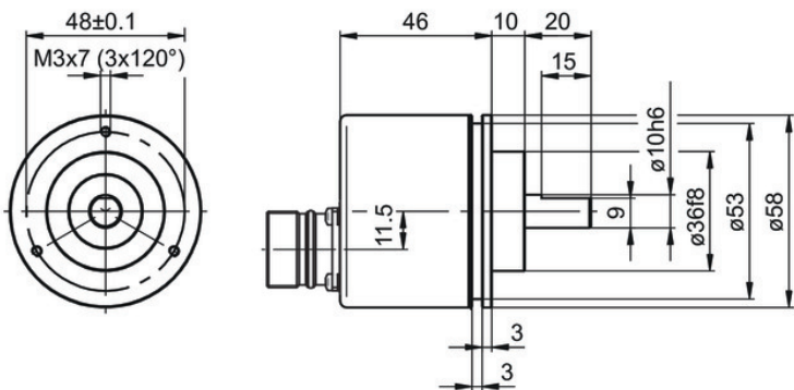
Connector M23, axial
