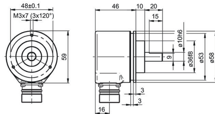
Connector M23, radial
